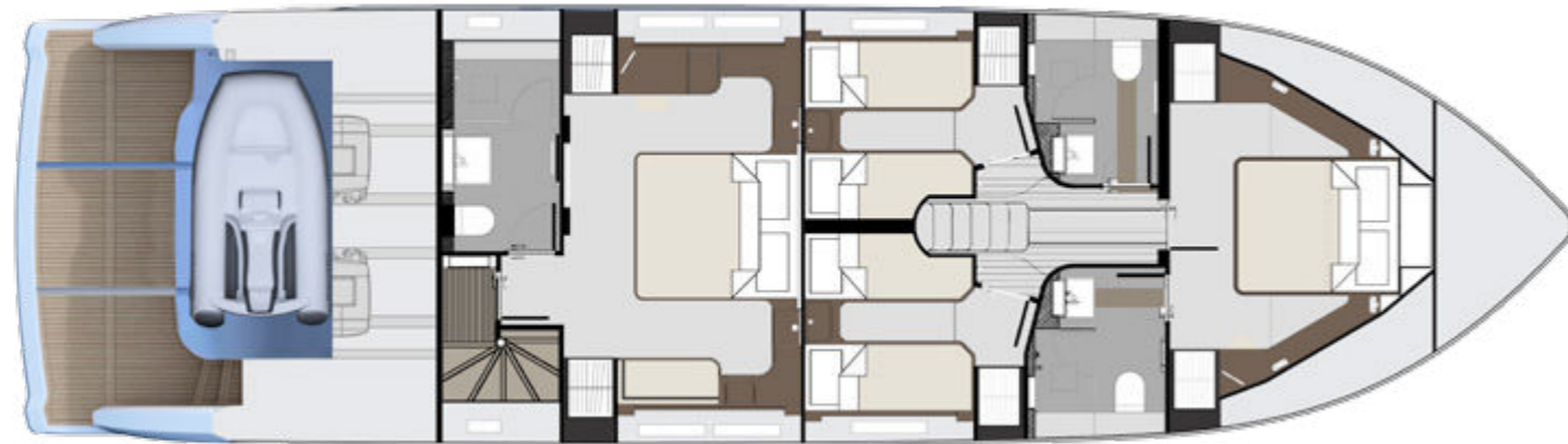
LOWER DECK
